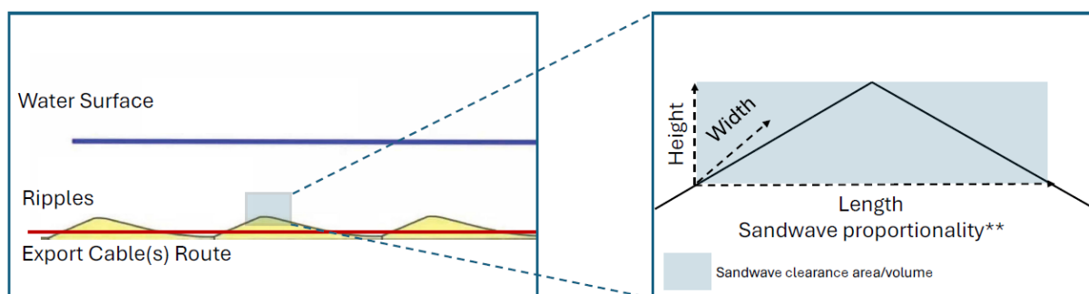
Figure 7: Sandwave profile
